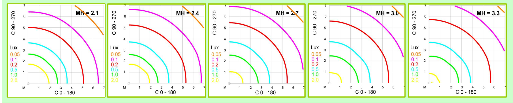
PSL10 Series STARLITE 6V 10W Tungsten Halogen - White Reflector Plate
